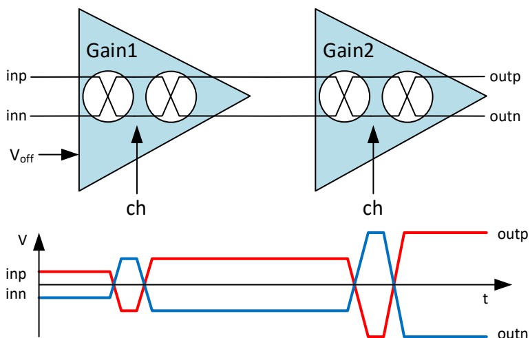
Figure 13: PGA Architecture
