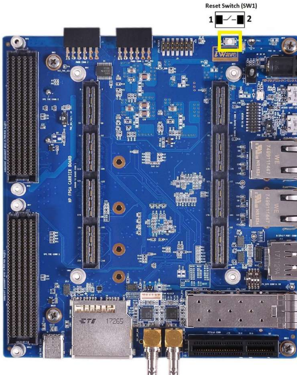
Figure 25: Reset Switch
