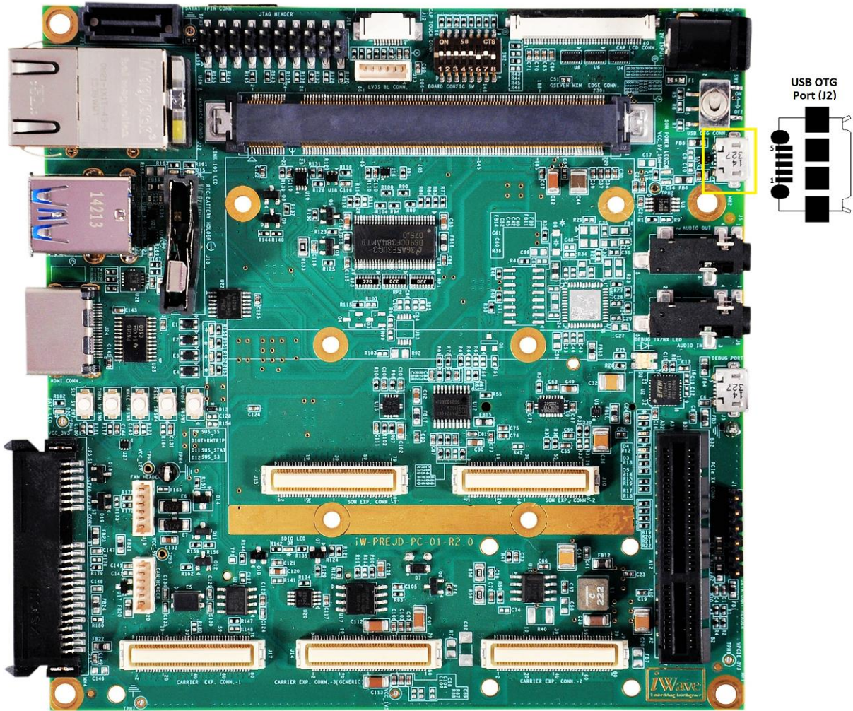
Figure 11: USB2.0 OTG
