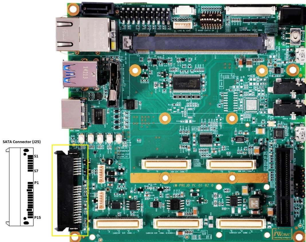
Figure 7: SATA Connector
