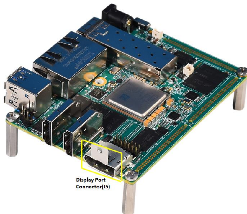
Figure 8: Display Port Connector
