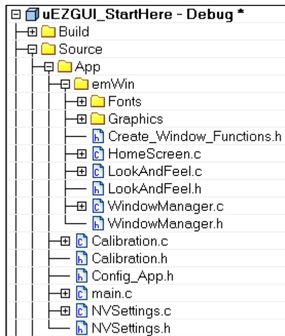
Figure 15: File Hierarchy
