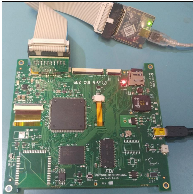
Figure 4: J-Link Connected to \mu EZ GUI
